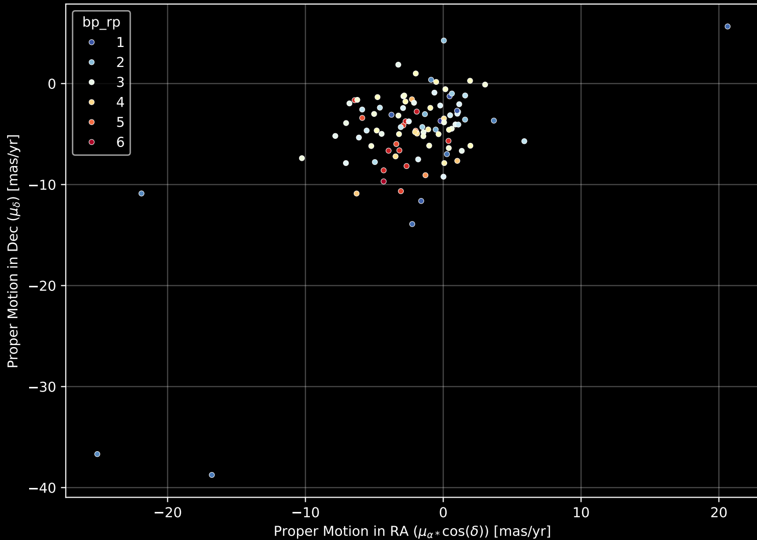
APOGEE DR17 Field: [004+04] Proper Motion Diagram (n= 98)
