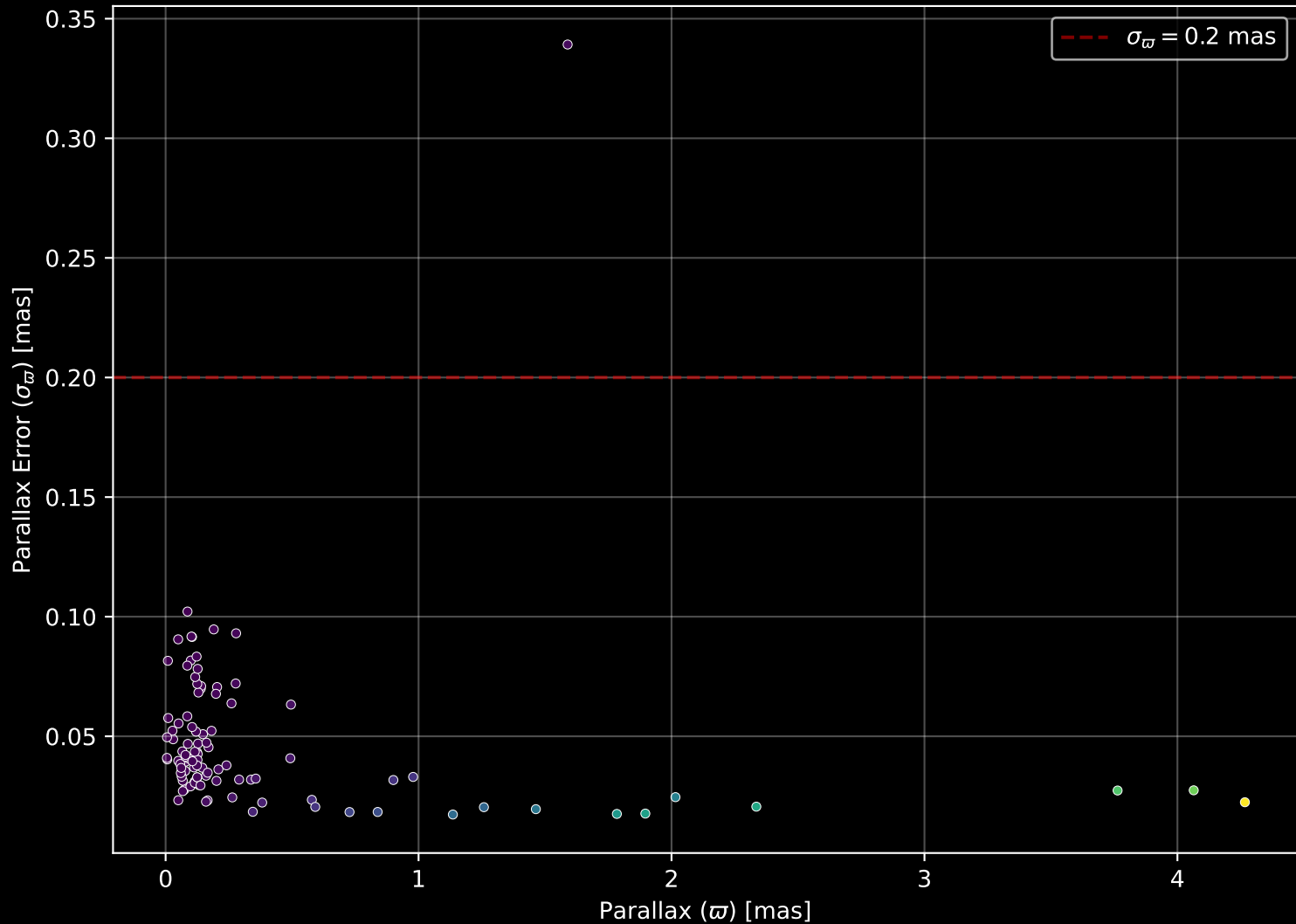
APOGEE DR17 Field: [004+04] Parallax Quality (n= 98)
