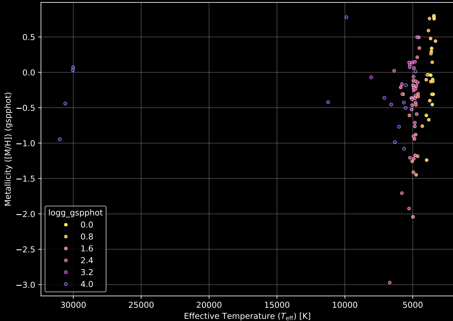
APOGEE DR17 Field: [004+04] Stellar Population Parameters (n= 98)
