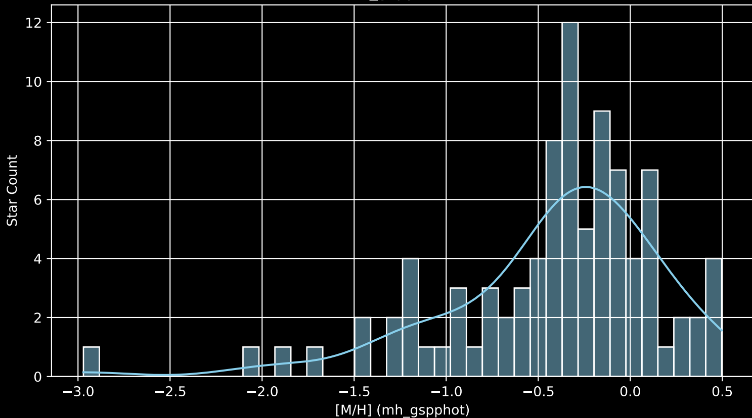
APOGEE DR17 Field: [004+04] [M/H] (mh_gspphot) (n= 91)
