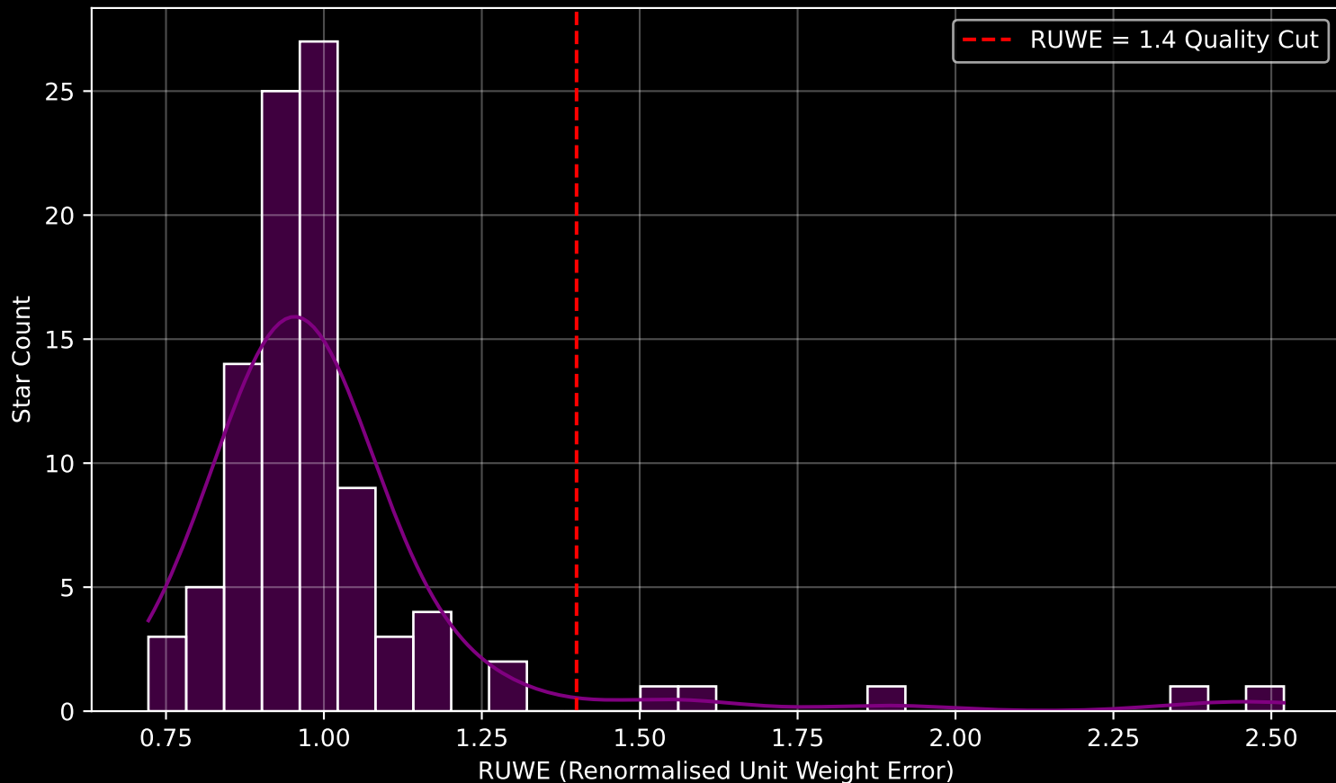
GAPOGEE DR17 Field [004+04] RUWE Distribution (n= 97)
